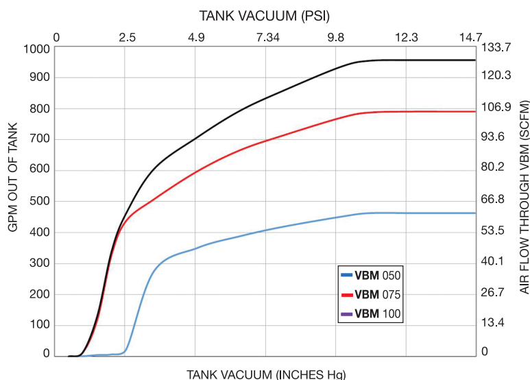
VBM AIR FLOW CHART - CALCULATED DATA AT 70°F
