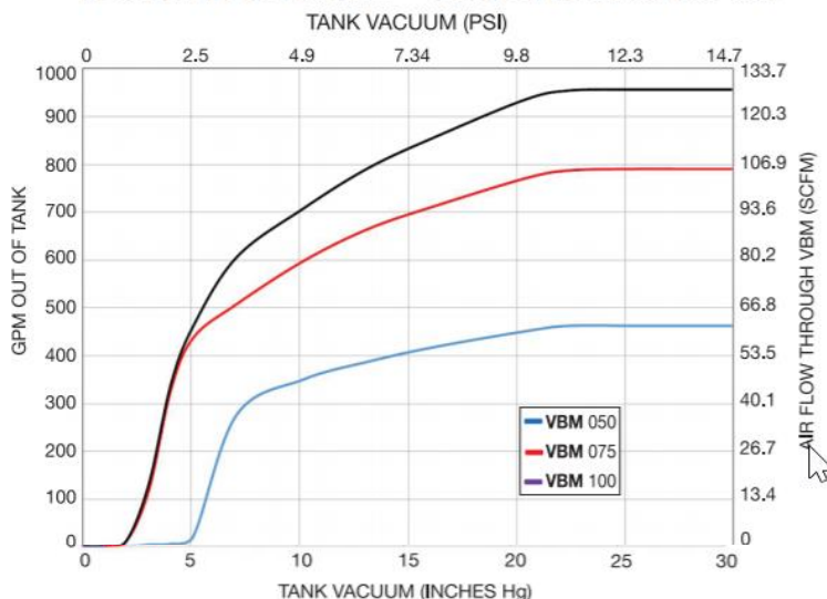
VBM AIR FLOW CHART - CALCULATED DATA AT 70°F
